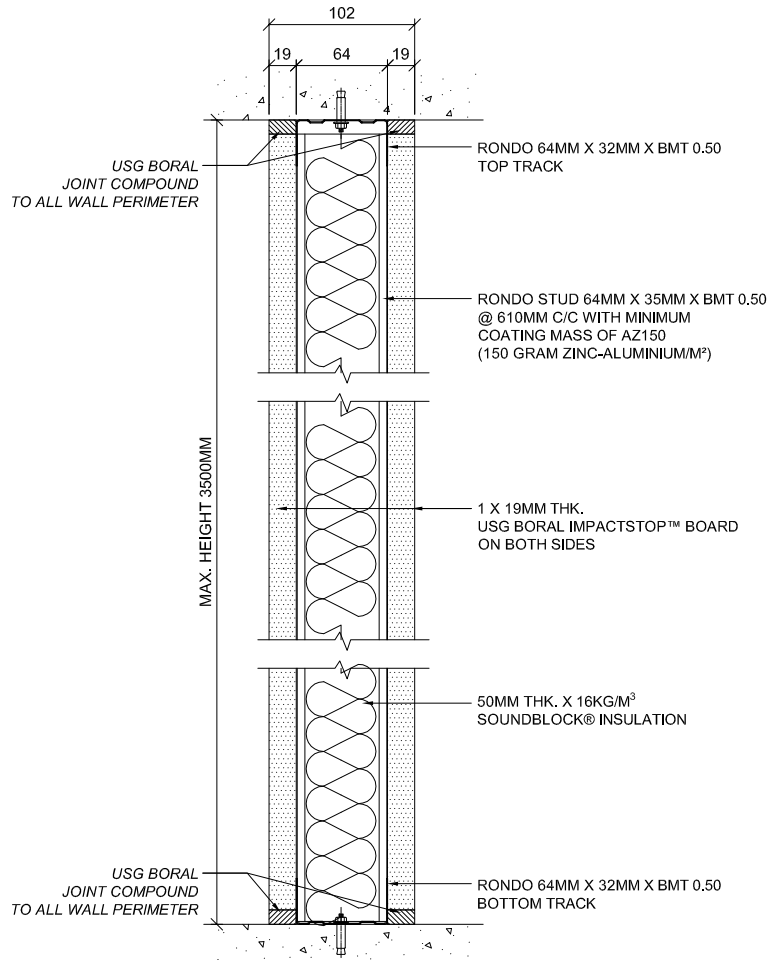
W1 SECTION NTS
