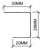
RONDO FURRING TRACK: PN 140 THICKNESS = BMT 0.50
