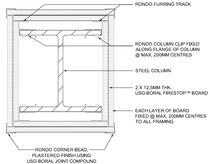
1HR FIRE RATED COLUMN PROTECTION SYSTEM
