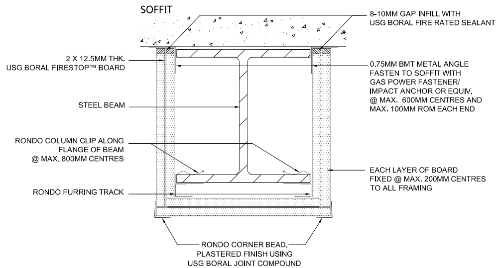
1HR FIRE RATED BEAM PROTECTION SYSTEM
