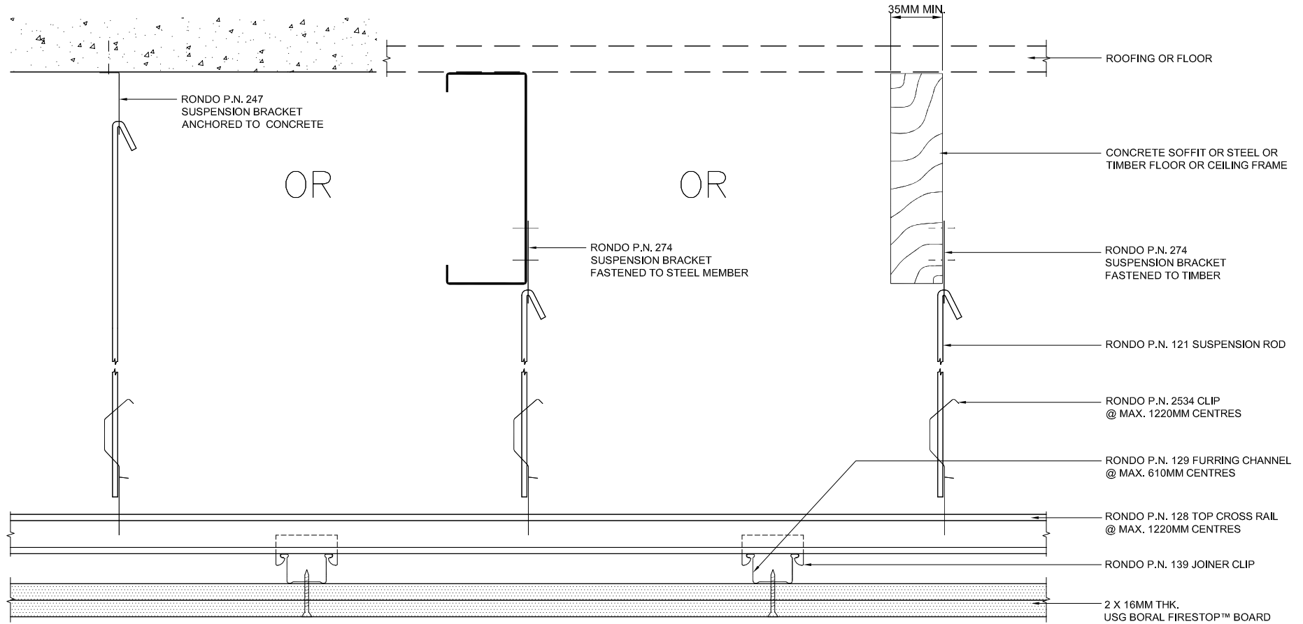
C1a NTS SUSPENSION CONNECTION SECTION DETAIL
