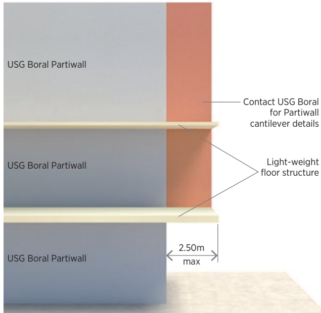
Figure 1: Cantilever Partiwall
