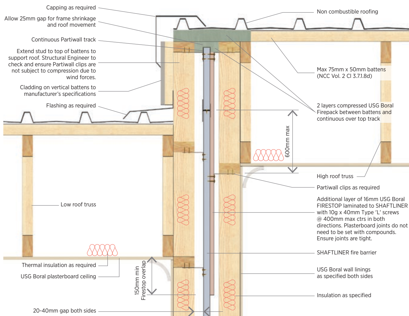
Figure 15: Staggered Roof Detail - Metal Roof - FRL 60/60/60
