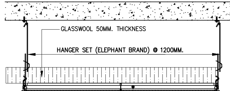
SECTION 2-2 SCALE 1 : 7.5
