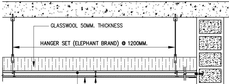
SECTION 1-1 SCALE 1 : 7.5
